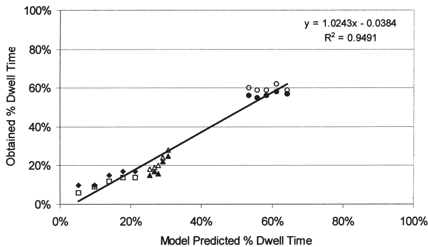
Figure 9. Model fit of communications experiment. Solid symbols = auditory, open symbols = visual; circles = IP, triangles = OW, squares = data link, diamonds = clipboard. The five communicative load points are not separately labeled but fall in monotonic order.
