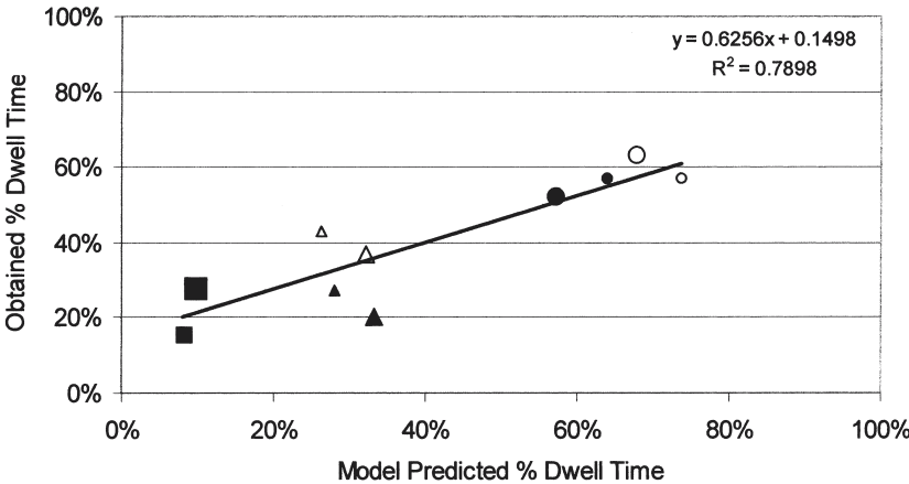
Figure 7. Model prediction versus scan (percentage dwell time) performance for the free-flight experiment. Squares = CDTI, triangles = OW, circles = IP; small = conflict, large = nonconflict; solid symbols = free flight, open symbols = baseline.
