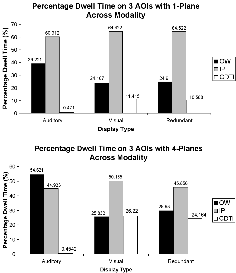
Figure 4. Top: Percentage dwell time on three areas of interest (AOIs) with one plane (low workload) across modality. Bottom: Percentage dwell time on three AOIs with four planes (high workload) across modality. (OW = outside world, IP = instrument panel, CDTI = cockpit display of traffic information.)
