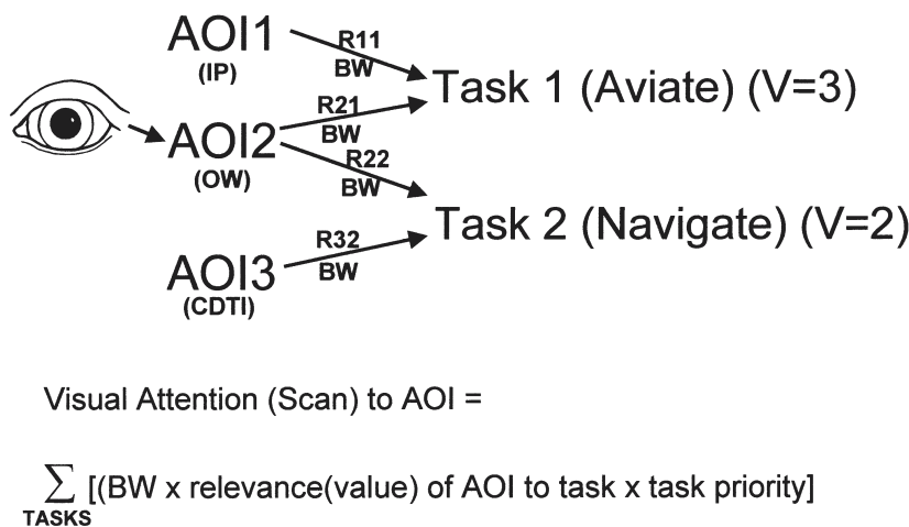
Figure 6. The expected value model of visual scanning or attention allocation. AOI = area of interest, IP = instrument panel, OW = outside world, CDTI = cockpit display of traffic information, BW = bandwidth, R_{xy} = relevance of AOI to Task Y. The higher the value (V) of a task, the more important that task is.
