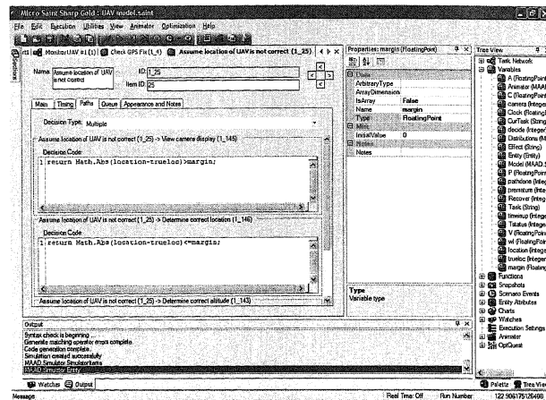
Figure 7 User interface in Micro Saint Sharp for defining task branching decision logic.
