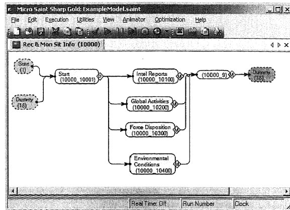
Figure 12 Second-level task network.
