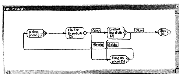
Figure 4 Task network model representing a human dialing a telephone.
