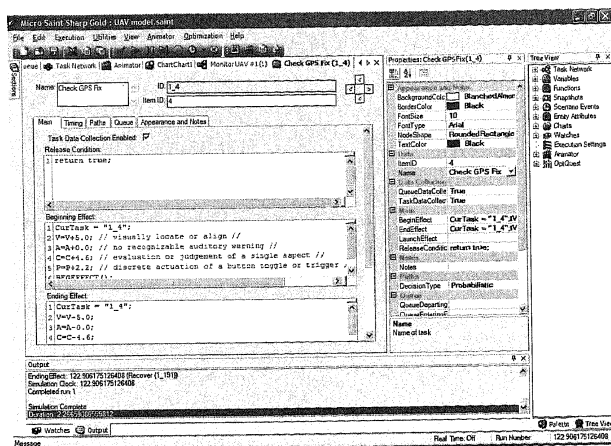
Figure 6 User interface in Micro Saint Sharp for providing input on a task.
