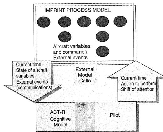
Figure 26 Integrated ACT-R/IMPRINT model.
