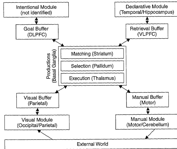
Figure 19 Modular view of ACT-R cognitive architecture.
