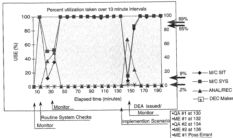
Figure 16 Model predictions of operator utilization over time.
