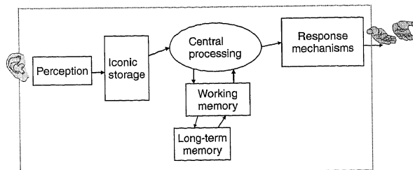
Figure 3 First-principle models of human performance.
