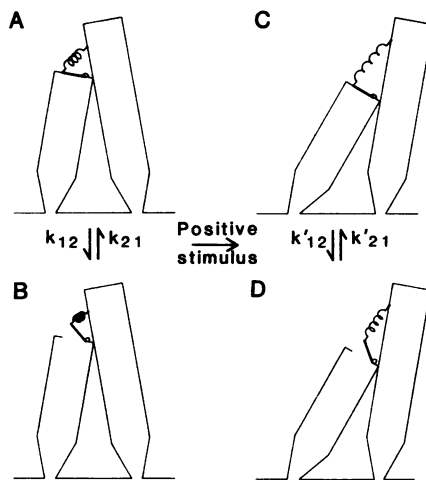
Fig. 5. A model for mechano-electrical transduction by hair cells. At any instant, each transduction channel at a stereocilium's tip may be either closed (A) or open (B). The relative values of the rate constants for channel opening and closing, k_{12} and k_{21} , respectively, determine the fraction of the transduction channels open in the undisturbed steady state. When the hair bundle is deflected with a positive stimulus (C and D), the values of the rate constants are altered; the opening rate constant ( k'_{12} ) is larger and the closing rate constant ( k'_{21} ) smaller than the original values. The new steady-state transduction current is therefore greater, and the cell is depolarized. Pushing the hair bundle in the opposite direction has a contrary effect on the rate constants, culminating in a hyperpolarizing response.
