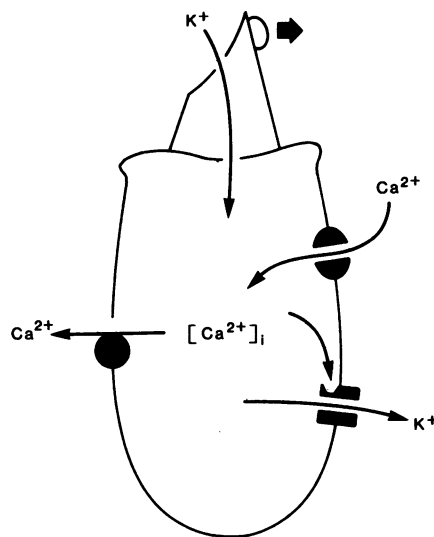
Fig. 7. A model for electrical resonance in hair cells. When the hair bundle is deflected, transduction channels open and positive ions, largely \text{K}^+ in vivo , enter the cell. The depolarization evoked by this transduction current activates voltage-sensitive \text{Ca}^{2+} channels. As \text{Ca}^{2+} ions flow into the cell, they augment the depolarization. At the same time, however, the influx of \text{Ca}^{2+} raises the intracellular concentration of this ion, [\text{Ca}^{2+}]_i , especially the local concentration just beneath the surface membrane. The high \text{Ca}^{2+} concentration brings into play the \text{Ca}^{2+} -sensitive \text{K}^+ channels. As \text{K}^+ exits through these pores, it begins to repolarize the membrane, thereby diminishing the activation of \text{Ca}^{2+} channels. The fluid bathing the apical surface of a hair cell characteristically has a much higher \text{K}^+ concentration than that contacting the basolateral cellular surface. As a consequence, \text{K}^+ can both enter and leave the cell passively. By the time the membrane potential is somewhat more negative than its steady-state value, the intracellular \text{Ca}^{2+} concentration is reduced by the sequestering of the ion within organelles and by its extrusion through ion pumps. As the \text{Ca}^{2+} -sensitive \text{K}^+ channels close, the cell returns to approximately its initial condition, and another cycle of the electrical resonance commences.
