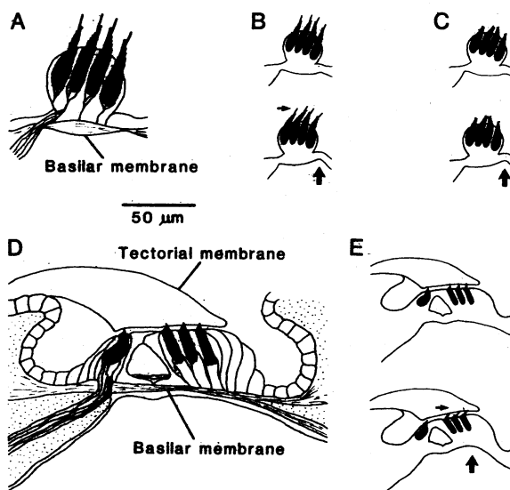
Fig. 3. Structures and operations of representative cochleas. Hair cells are shown solid black. (A) A schematic cross-section through the cochlea of the alligator lizard ( Gerrhonotus multicarinatus ), which contains the organ's longest freestanding hair bundles. (B) When the lizard's ear is stimulated by low-frequency sound, differences in fluid pressure across the basilar membrane cause it to move vertically. As the hair cells upon the basilar membrane sway laterally, the inertia and hydrodynamic resistance of the hair bundles cause them to be bent; this deflection in turn excites the hair cells. (C) Because of their lesser inertia and drag, the short hair bundles at the organ's opposite end do not re-
