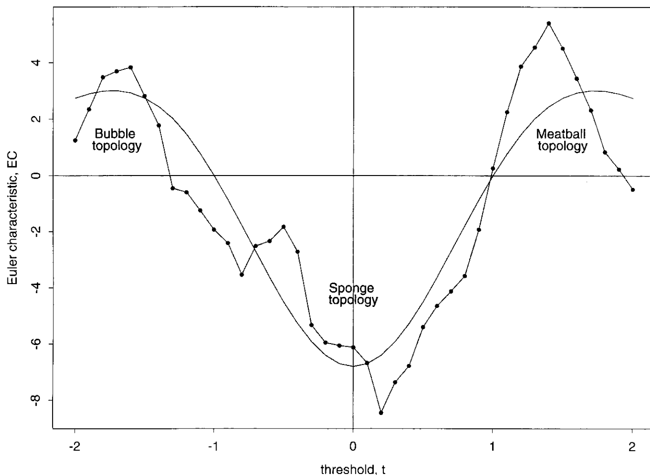
Figure 4. Plot of the observed EC of the set of high-density regions of the real galaxy data (points), and the expected EC from the formula (curve) for a Gaussian random-field model, plotted against the density threshold. The observed and expected are in reasonable agreement, confirming the Gaussian random field model: high thresholds produce a "meatball" topology (Fig. 2a); medium thresholds produce a "sponge" topology (Fig. 2b), and low thresholds produce a "bubble" topology (Fig. 2c).
