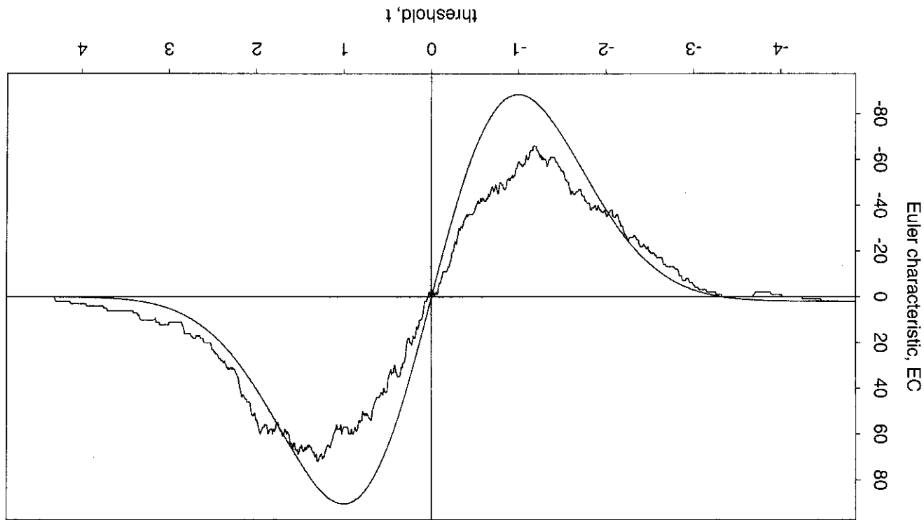
Figure 11. Plot of the observed EC of excursion sets of the anomalies in the cosmic microwave background radiation (jagged line), and the expected EC from the formula (smooth line) if there are no real anomalies. The observed microwave background radiation produces an EC curve similar in shape to that expected, but somewhat lower and spread more in the tails—evidence that some of the anomalies are real and not just due to random noise. This discrepancy points to a Gaussian random field model for the anomalies, with a larger standard deviation and a larger smoothness than the background noise.
