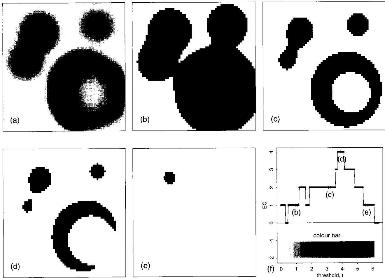
Figure 9. The EC of the excursion set of a random field in 2-D is the number of maxima ( M ) – saddles ( S ) + minima ( m ) of the field inside the excursion set. For an artificial image (a), the EC of the excursion set for a low threshold (b) at t = 1 is EC = 4 - 4 + 1 = 1 ; (c) at t = 2.8 the local minimum disappears, leaving a hole, and EC = 4 - 2 + 0 = 2 ; (d) at t = 3.2 the hole breaks open leaving components with just one local maximum in each, and EC = 4 - 0 + 0 = 4 ; (e) at t = 5.6 , just below the global maximum, EC = 1 - 0 + 0 = 1 ; above the global maximum the EC is 0, so that for high thresholds the expected EC approximates the p value of the global maximum; (f) is a plot of the EC against the threshold, t .
