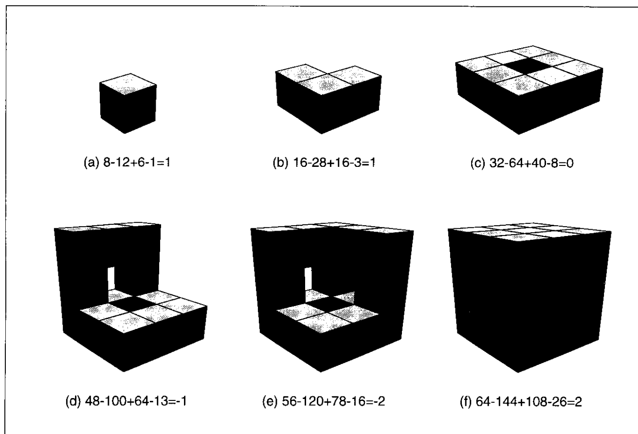
Figure 1. The Euler characteristic (EC) of a solid is the number of vertices – edges + faces – polyhedra. For a single polyhedron (a) or several joined together (b), the EC = 1; if there is a hole in the solid (c) the EC = 0; and the EC decreases by 1 for each extra hole (d, e); in (f) the central cube is missing so the solid is hollow, in which case the EC = 2.
