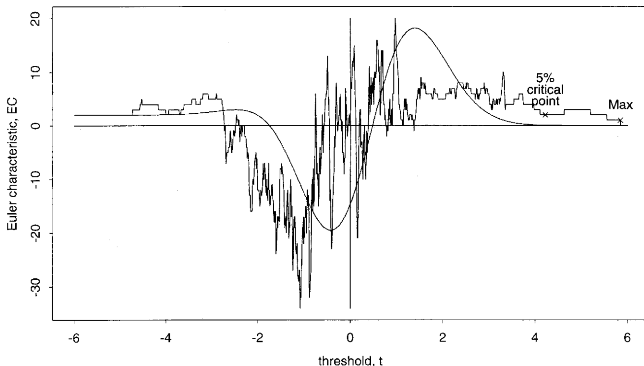
Figure 12. Plot of the observed EC of the set of high-Z regions for the PET data (jagged line) and the expected EC from the formula (smooth line) if there is no activation due to the linguistic task, plotted against the threshold t . The most interesting part is when t > 3 , showing more EC than expected, confirming that some components of the excursion set are due to the linguistic task and not the random noise. In particular, at t = 3.3 we expect an EC of 1, but we observe 4 (visible in Fig. 9g); at the 5% critical value of t = 4.22 , we expect .05 but we observe 2 components (visible in Fig. 9h).
