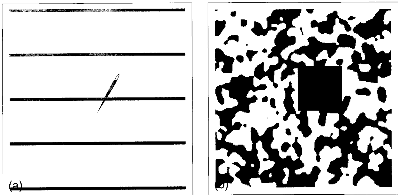
Figure 10. A generalization of Buffon's needle is used to find the formula for the expected EC of the excursion set; (a) a needle is thrown at random onto the floor; if the length of the needle is the same as the separation of the cracks in the floor boards, then the probability of the needle crossing a crack is 2/\pi ; (b) replace the needle with the search region (square shape shown in 2-D) and the cracks with the excursion set of a random field, extended on all sides; the Kinematic Fundamental Formula gives the expected EC of the points in common (black), which leads eventually to the formula we want.
