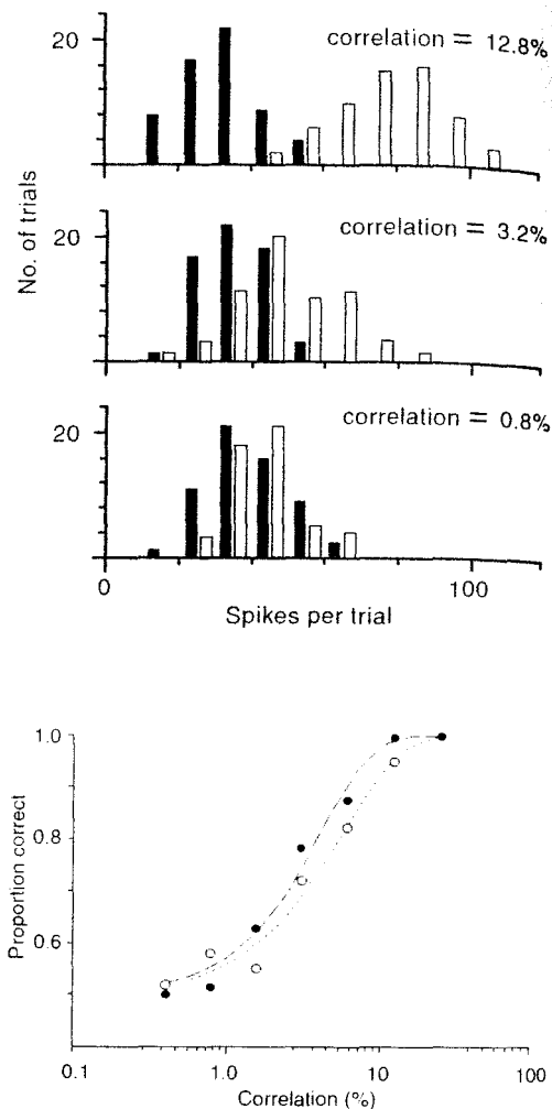
FIGURE 10.1 ■ Physiological and Psychophysical Data Obtained Simultaneously from a rhesus monkey. a . The responses of a directionally selective MT neuron at three different motion correlations spanning physiological threshold. The hatched bars represent responses to motion in the neuron's preferred direction; the solid bars indicate responses to motion in the null direction (180° opposite to the preferred). Sixty trials were performed in each direction for each of the three correlation levels. Response distributions for a range of correlation levels were used to compute a "neurometric" function that characterized the neuron's sensitivity to the motion signal and could be compared with the psychometric function computed from the monkey's behavioural responses. b . Comparison of simultaneously recorded psychometric and neurometric functions. Psychophysical performance of the monkey, \circ ; performance of the neuron \bullet . Psychophysical performance at each correlation is given by the proportion of trials on
