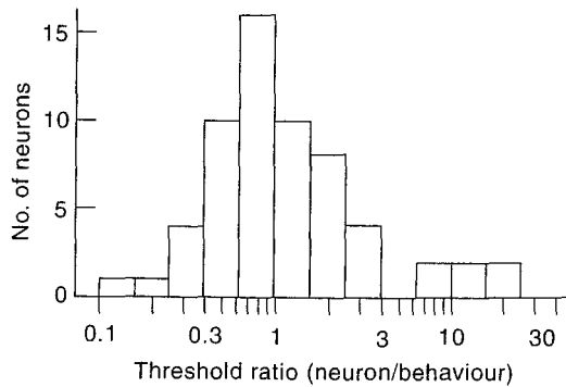
FIGURE 10.2 ■ Comparison of Psychophysical and Physiological Thresholds Obtained for 60 MT Neurons in Two Rhesus Monkeys. The frequency histogram shows the distribution of the ratio of the physiological threshold to the psychophysical threshold for all the neurons for which we obtained data. A value of 1 represents perfect correspondence between psychophysical and physiological thresholds; values < 1 indicate that the physiological threshold was lower than the physiological threshold, whereas values > 1 indicate the converse. The directional preferences of the 60 neurons were roughly uniformly distributed and there was no reliable association between a neuron's direction or speed preference and its threshold relative to the perceptual threshold.
