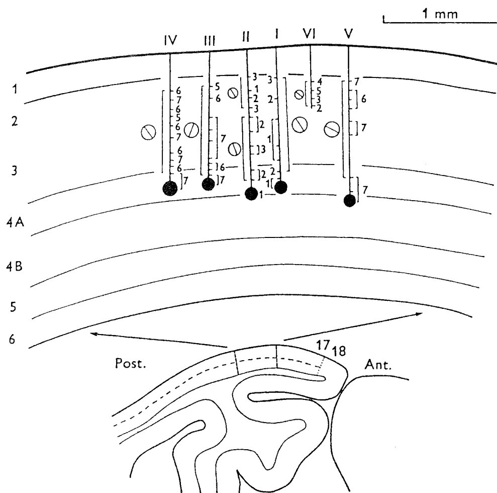
FIGURE 7.11 ■ Six Closely Spaced Parallel Penetrations through Rhesus Striate Cortex Made to Determine the Layer in which Background and Some Units Lacked Orientation Specificity, and in which most Cells were Driven by One Eye Exclusively. Lesion made in these regions are indicated by black circles. Lines within the open circles indicate optimum stimulus orientation. Numbers to right of each penetration refer to ocular dominance group of each isolated unit.
