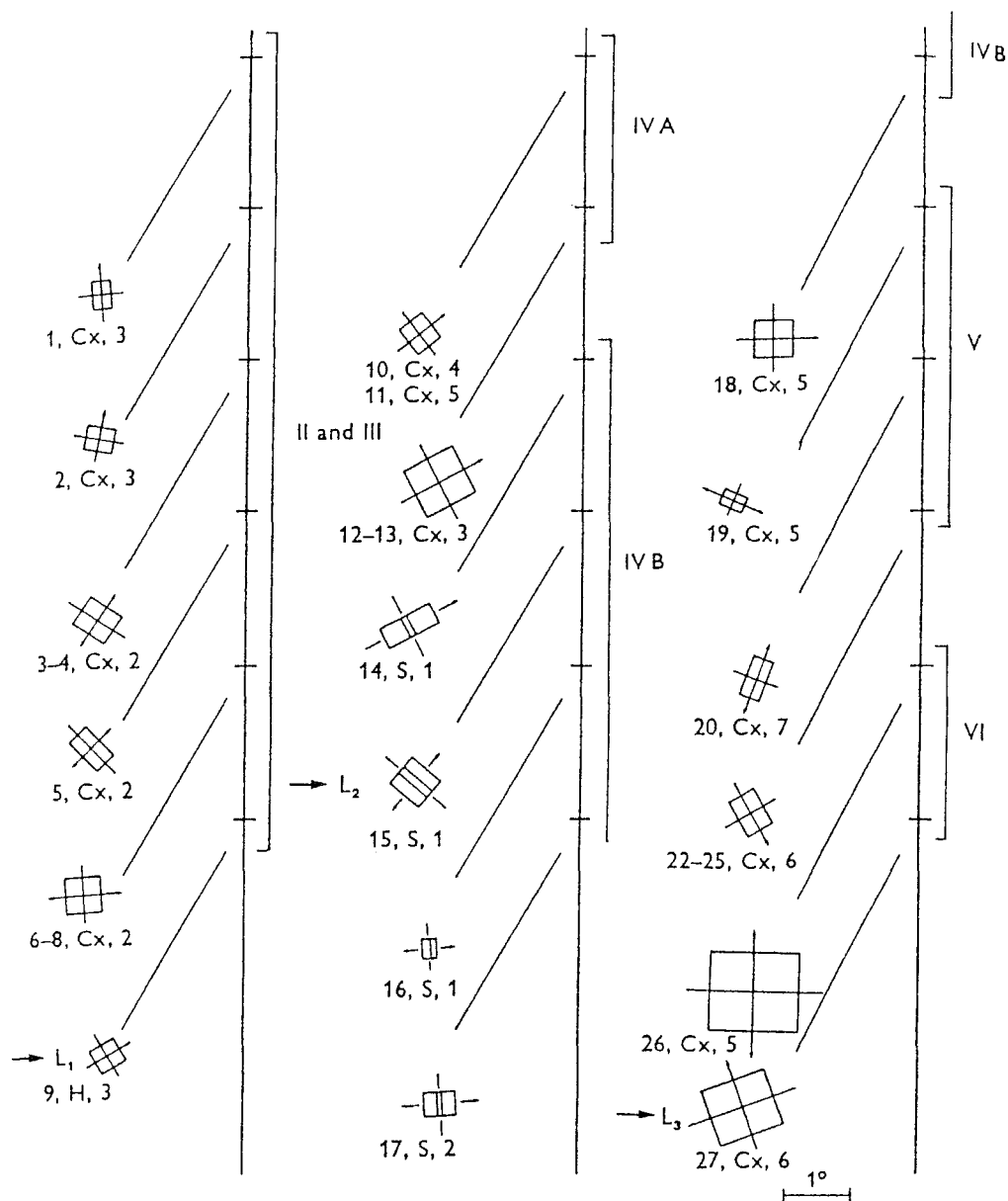
FIGURE 7.8 ■ Receptive-field Diagrams for Units Recorded in the Penetration of Fig. 7. Approximate positions and shapes of each field, referred to the fovea, are indicated by rectangles. Foveas are indicated separately for each field by the short horizontal lines intersecting the three long vertical lines. Responses to a moving line are shown for every field by arrows; a single arrowhead indicates strong directional preference. Square brackets refer to cortical layers. For each field the first number is the unit number; S, Cx and H mean simple, complex and hypercomplex; the last number refers to ocular-dominance groups. Cells of group 1 were driven only by the contralateral eye; for cells of group 2 there was marked dominance of the contralateral eye; for group 3, slight dominance. For cells in group 4 there was no obvious difference between the two eyes. In group 5 the ipsilateral eye dominated slightly; in group 6 markedly, and in group 7 the cells were driven only by the ipsilateral eye.
