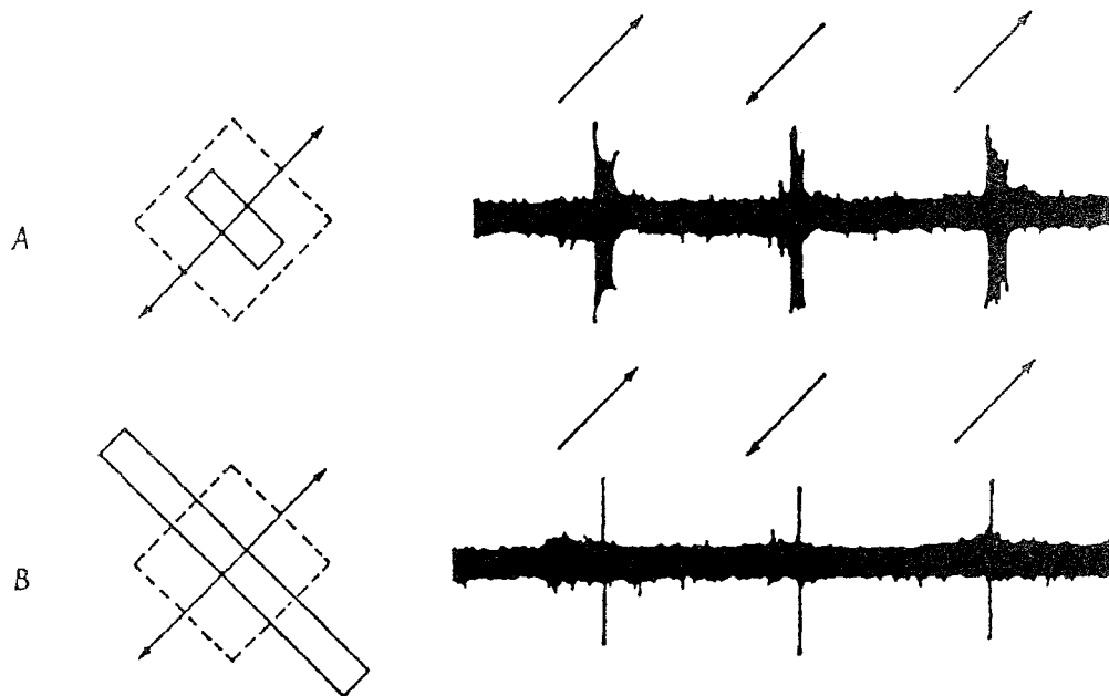
FIGURE 7.4 ■ Hypercomplex Cell Recorded from Right Striate Cortex, Layer II. A: stimulus of left eye by moving slit within activating region ( \frac{1}{4} \times \frac{3}{8}^\circ ); B: similar stimulation with slit extending beyond activating region. Background, log 0.0 cd/m 2 ; stimulus, log 1.3 cd/m 2 . Duration of each record 10 sec.
