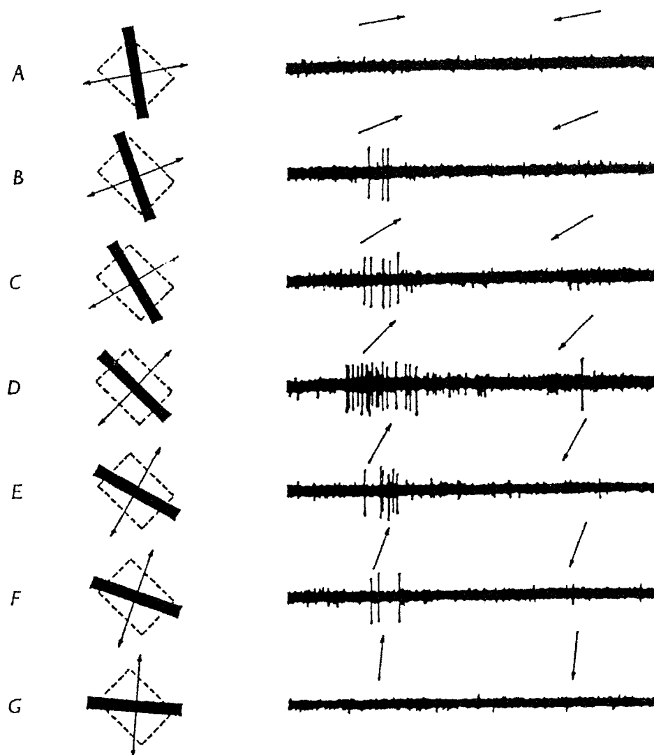
FIGURE 7.2 ■ Responses of a Complex Cell in Right Striate Cortex (layer IV A) to Various Orientations of a Moving Black Bar. Receptive field in the left eye indicated by the interrupted rectangles; it was approximately 3/8 \times 3/8^\circ in size, and was situated 4^\circ below and to the left of the point of fixation. Ocular-dominance group 4. Duration of each record, 2 sec. Background intensity 1.3 \log_{10} \text{ cd/m}^2 , dark bars 0.0 \log \text{ cd/m}^2 .
