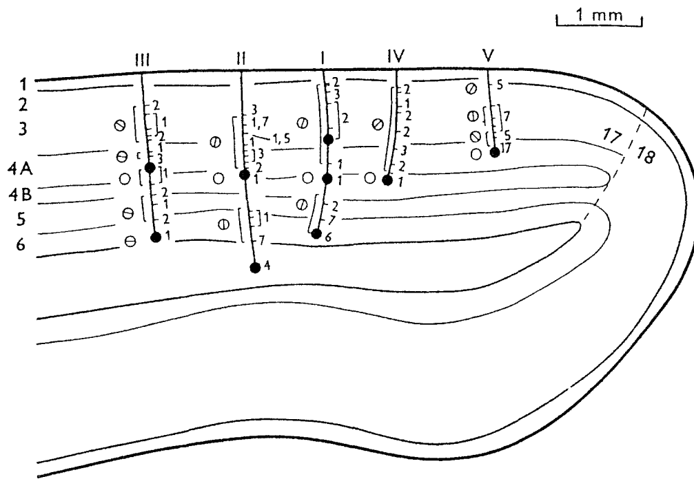
FIGURE 7.12 ■ Five Close-spaced Penetrations in Rhesus Area 17. Open circles indicate a lack of background orientation specificity; other conventions as in Fig. 11.
