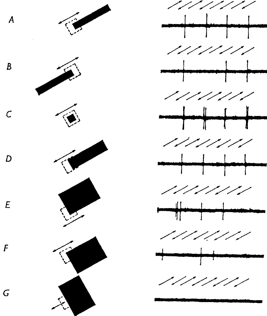
FIGURE 7.3 ■ Responses of a Hypercomplex Cell from Layer III of Monkey Striate Cortex. (This was cell 9 in Figs. 7 and 8). 'Activating' portion of receptive field ( 3/8 \times 3/8^\circ ) is outlined by interrupted lines. Stimulus of this region by a moving edge activates cell (A–D). Below this region, and to some extent above it, are regions appropriate stimulation of which suppresses the response to an edge (E–G). Duration of each record 5 sec. Stimulus intensities as in Fig. 2.
