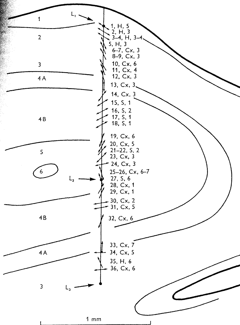
FIGURE 7.10 ■ Reconstruction of an Oblique Penetration through Striate Cortex of Spider Monkey. This experiment indicates laminar groupings of cells according to complexity, and aggregation according to orientation, directionality of movement, and ocular-dominance. As in Fig. 8, 19 Cx 6 means 'Unit 19, complex, ocular-dominance group 6'.
