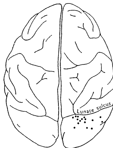
FIGURE 7.1 ■ Recording Sites for the Sixteen Rhesus Experiments. Diagram of monkey brain viewed from above; anterior is up. Many of the dots represent several closely spaced penetrations in a single monkey. Several deep penetrations went into buried folds of striate and non-striate cortex.
