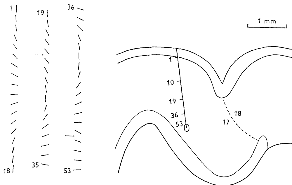
FIGURE 7.9 ■ Reconstruction of a Penetration Through Striate Cortex about 1 mm from 17–18 Border, Near Occipital Pole of Spider Monkey. To the left of the figure the lines indicate orientations of columns traversed; each line represents one or several units recorded against a rich unresolved background activity. Arrows indicate reversal of directions of shifts in orientation. Histological section through first part of this penetration is shown in Pl. 2.
