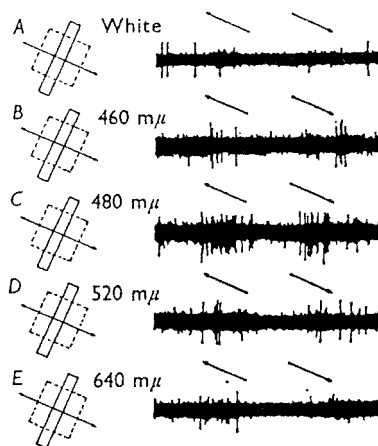
FIGURE 7.5 ■ Complex Cell with Colour Coded Properties Recorded in Layer II of Striate Cortex. Responses to movement of optimally oriented slits of white light and monochromatic light at various wave-lengths. Monochromatic light made by interposing interference filters in a beam of white light: stimulus energies are greatest for A, and progressively less for E, D, C, and B. None of the responses was improved by lowering the intensity. Size of receptive field 1\frac{1}{2} \times 1\frac{1}{2}^\circ . Ocular dominance group 1. Background and white stimulus intensities as in Fig. 4. Time for each record 5 sec.
