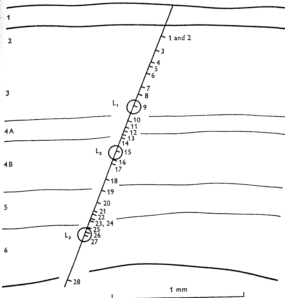
FIGURE 7.7 ■ Positions of Twenty-eight Units Recorded in a Single Penetration through Rhesus Striate Cortex. Positions of three lesions ( L_1 – L_3 ) are indicated by circles (see also Pl. 1 and Fig. 8).
