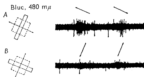
FIGURE 7.6 ■ Same Cell as Fig. 5. Responses to Two Orthogonal Stimulus Orientations at 480 mμ.
