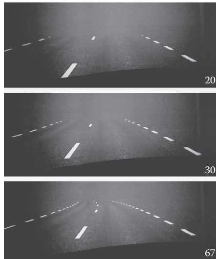
FIGURE 2.5 Examples of three different simulated driving preview distances. Edge lines are visible out to 20, 30, and 67 m, respectively. (Source: COST 331, 1999.)
