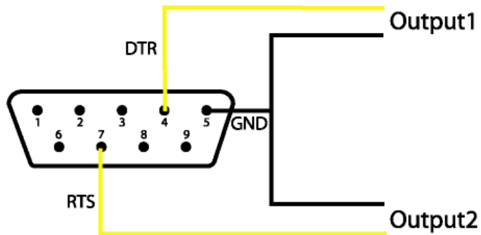
Serial port connector (solder bucket view)
